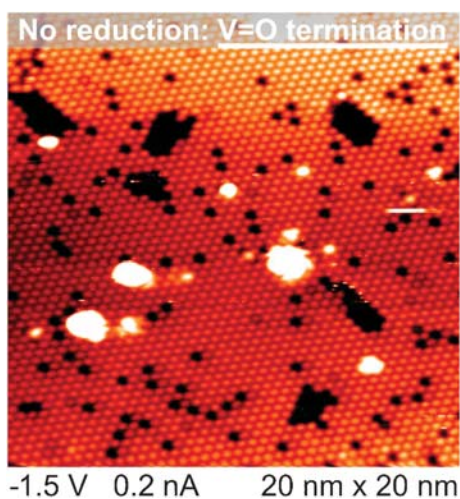
Fig. 6 V_2O_5 (0001) surface of a vanadium sesquioxide film grown on Au(111) as imaged with the STM (atomic resolution) (reproduced with permission from ref. 85. Copyright 2006, Springer).
