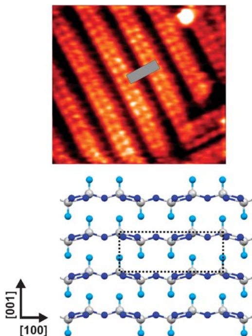
Fig. 5 Top: STM image of a V_2O_5 (010) film formed by the oxidation of 5.2 MLE V/Au(111). 5 \text{ nm} \times 2.8 \text{ nm} , 3 V, 0.2 nA. The surface unit cell is indicated by a grey parallelogram. Bottom: Schematic representation of a V_2O_5 single crystal in its stacking along the (010) direction. Grey circles represent V atoms, light and dark blue circles represent O atoms. 88,209–211 (Reproduced with permission from ref. 88; Copyright 2008, American Chemical Society.)
